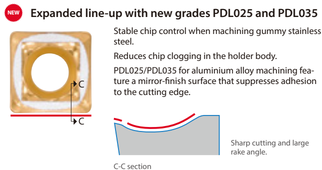
SM chipbreaker for stainless steel and aluminium alloy machining
