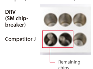
Comparison of remaining chips (in-house evaluation)
