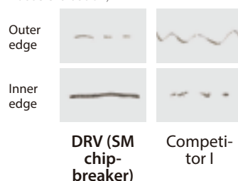
Chip control comparison (In-house evaluation)
